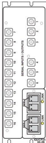
BOARD IQUCP25 8 SDI IN 8 SDI OUT
